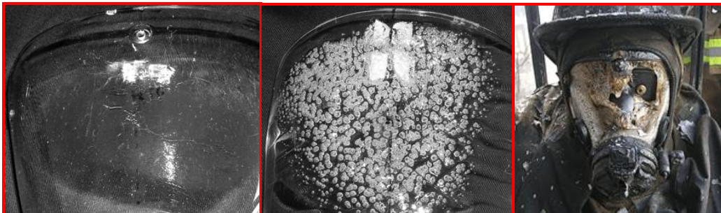
Photos showing examples of crazing (left), bubbling (center), and deformation from softening and bubbling (right) of facepiece lenses.
